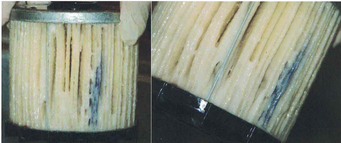
The waxy deposits in this plugged fuel filter were laboratory tested for Pour Point - the result was + 62°F. This indicates the deposit material plugging the filter is paraffin.
